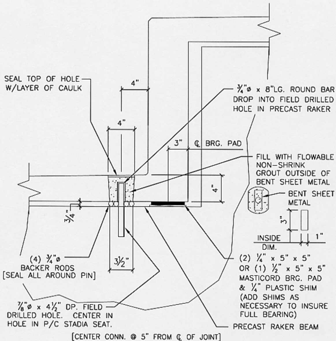
STADIA SEAT TO PRECAST RAKER BEAM FREE CONNECTION OPTION: A CAST-IN INSERT MAY BE SUBSTITUTED FOR A FIELD DRILLED HOLE.
